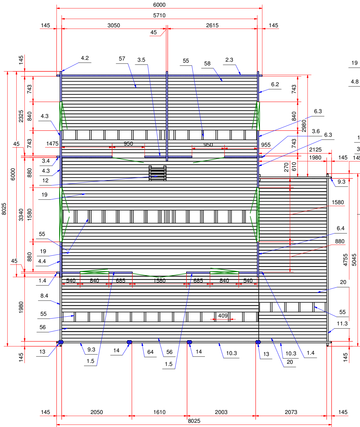
(house plan)
