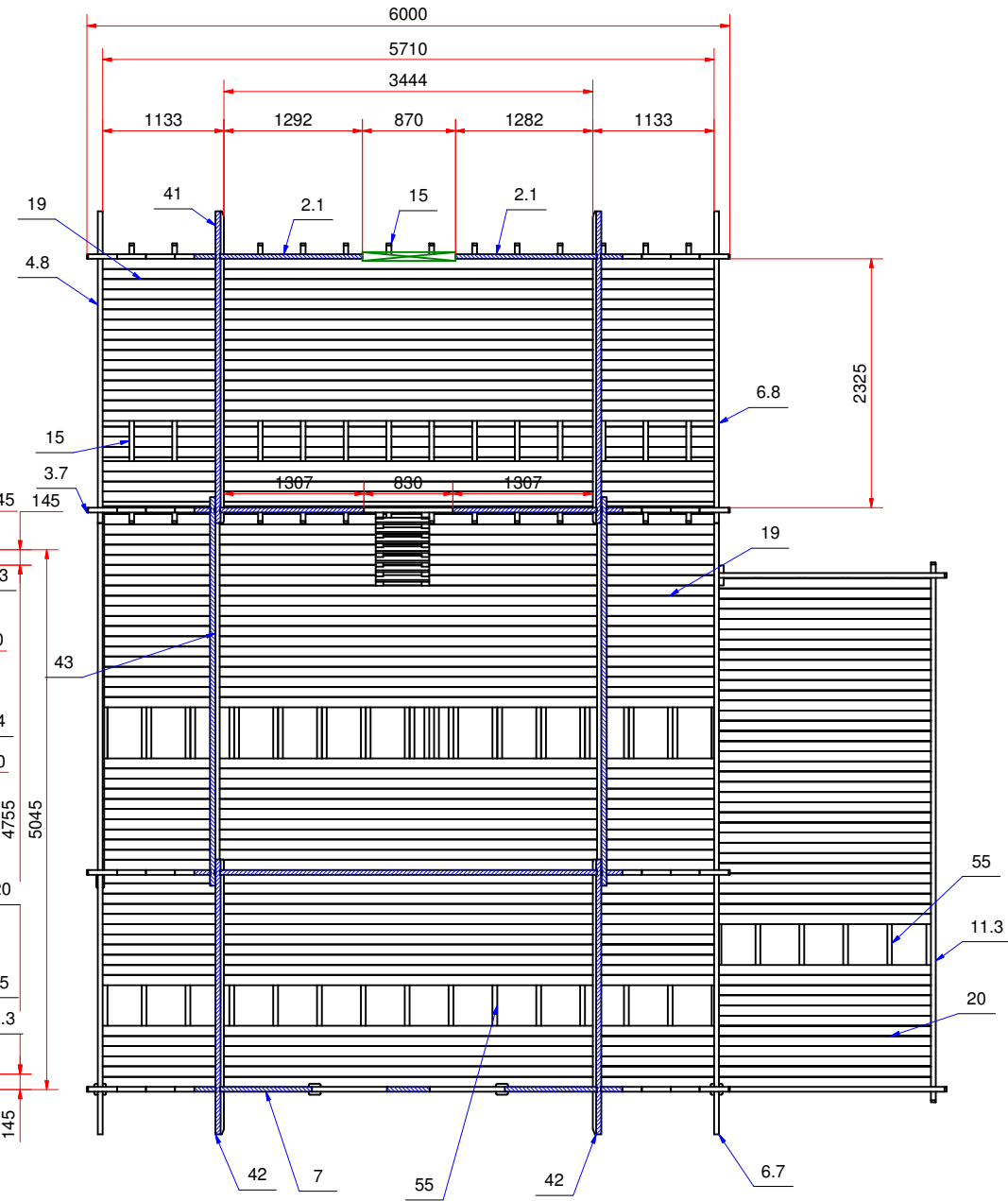
(house plan)
