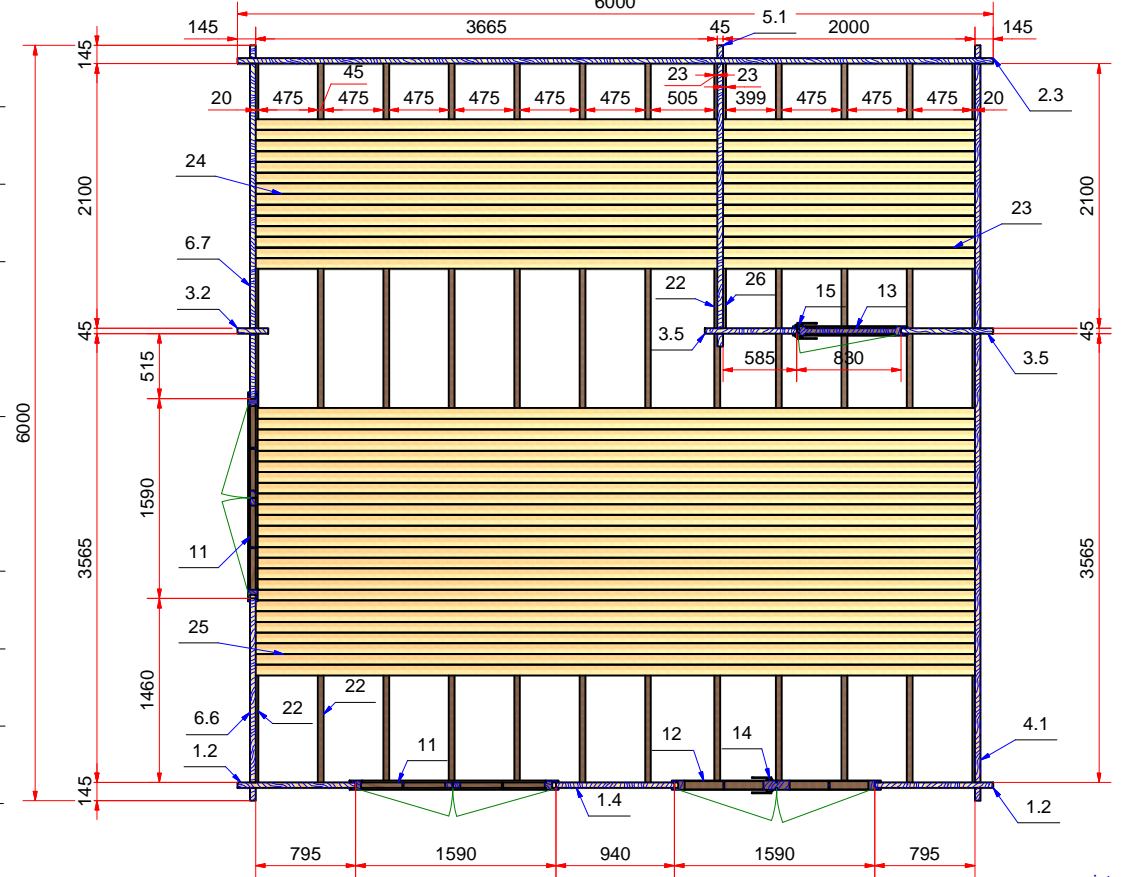
(house plan)
